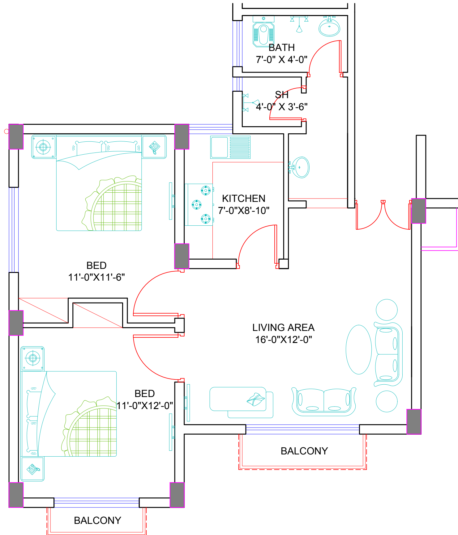
SINGLE UNIT PLAN
